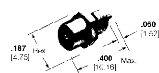
Part No. 413020-1
