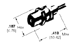
.047 [1.19] Semi-Rigid Cable - Part No. 413024-1
