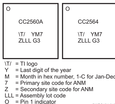
Figure 8-1. Chip Markings
