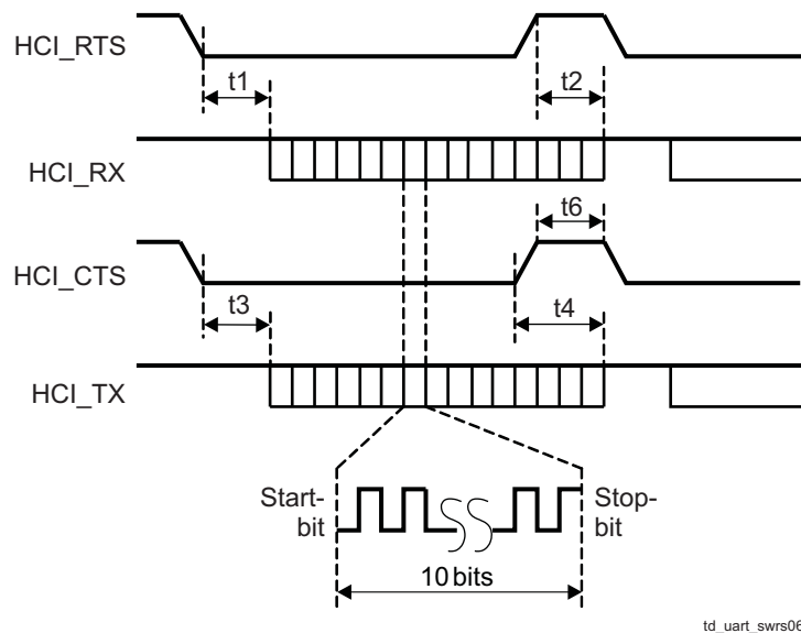
Figure 5-1. UART Timing
