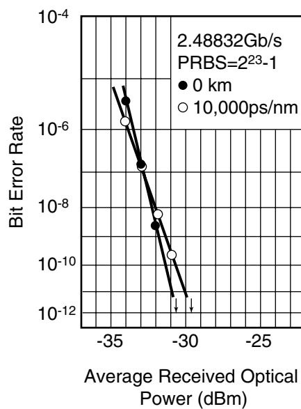
Fig. 8 Transmission Characteristics
