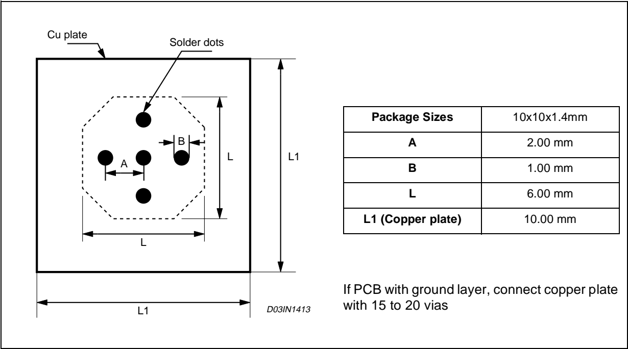
Figure 24. Soldering Information
