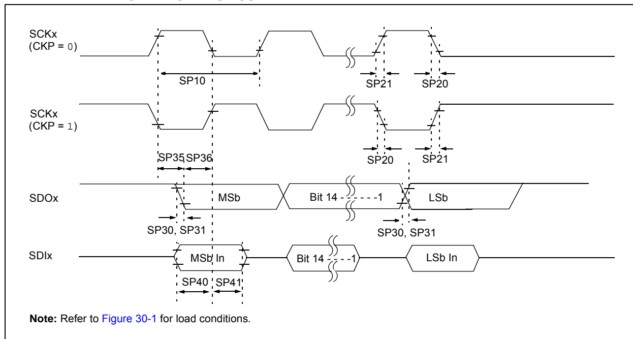
FIGURE 30-17: SPI2 MASTER MODE (FULL-DUPLEX, CKE = 0, CKP = x, SMP = 1) TIMING CHARACTERISTICS
