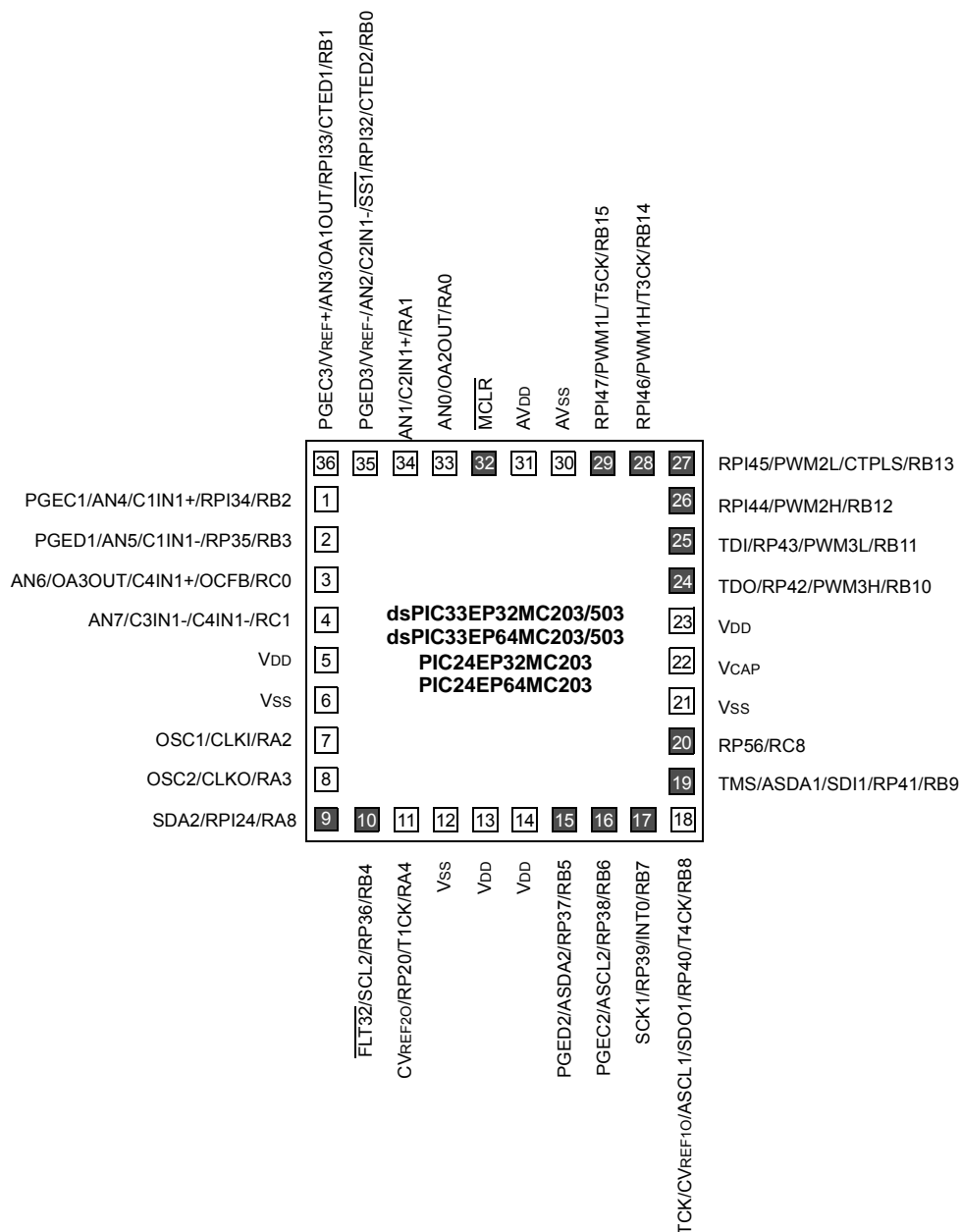
36-Pin VTLA (3)
