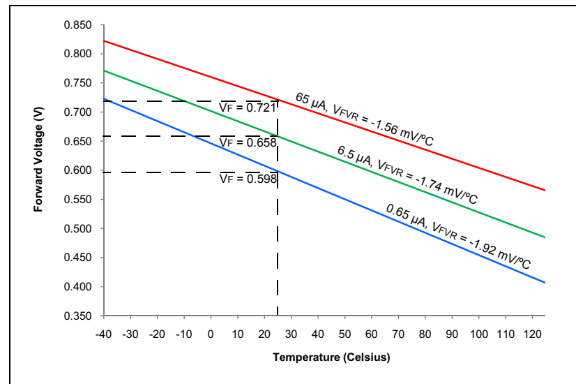
FIGURE 31-11: TYPICAL CTMU TEMPERATURE DIODE FORWARD VOLTAGE
