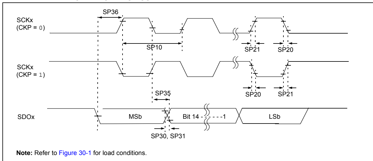
FIGURE 30-23: SPI1 MASTER MODE (HALF-DUPLEX, TRANSMIT ONLY) TIMING CHARACTERISTICS
