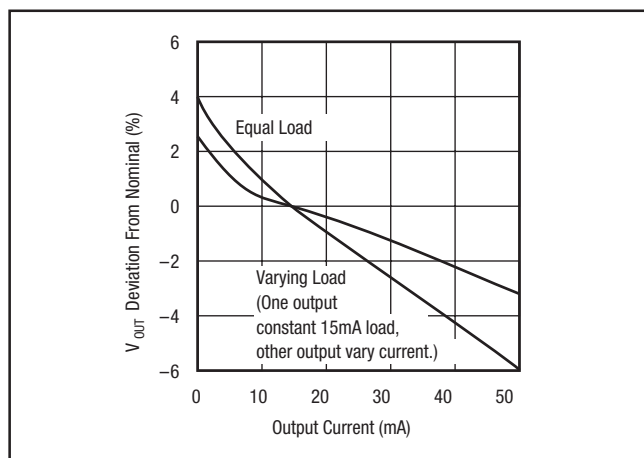
FIGURE 1. Load Regulation.
