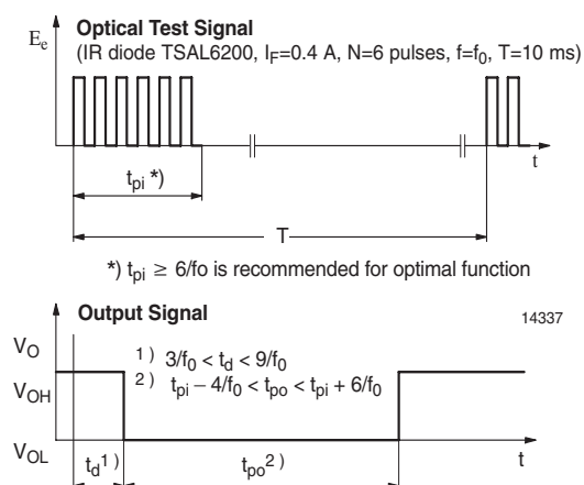
Figure 1. Output Function
