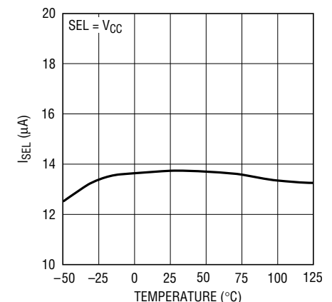
I_{\text{SEL}} vs Temperature
