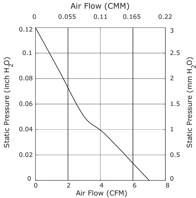
CFM-4010V-058-206
