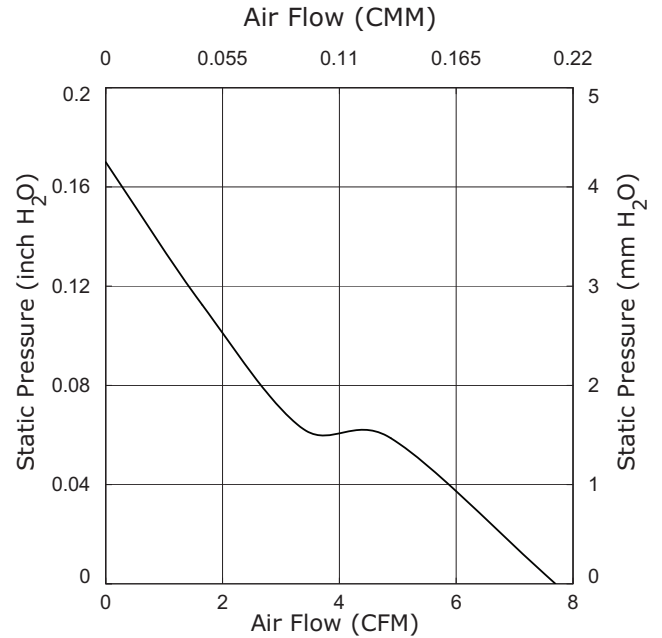
CFM-4020V-160-210
