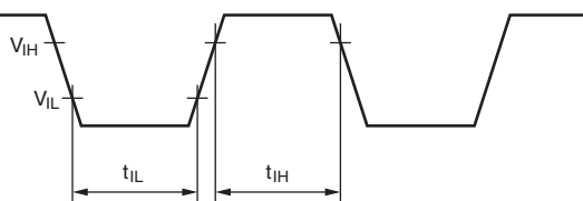
Figure 21.3 Input Timing
