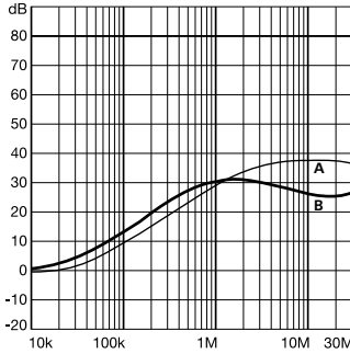
FN 9280BE Series | Typical filter attenuation | Per CISPR 17; A = 50Ω/50Ω sym; B = 50Ω/50Ω asym
