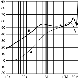
FN 9280E Series | Typical filter attenuation | Per CISPR 17; A = 50Ω/50Ω sym; B = 50Ω/50Ω asym
