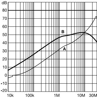
FN 9280 Series | Typical filter attenuation | Per CISPR 17; A = 50Ω/50Ω sym; B = 50Ω/50Ω asym
