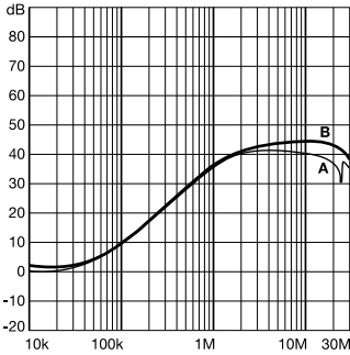
FN 9280B Series | Typical filter attenuation | Per CISPR 17; A = 50Ω/50Ω sym; B = 50Ω/50Ω asym
