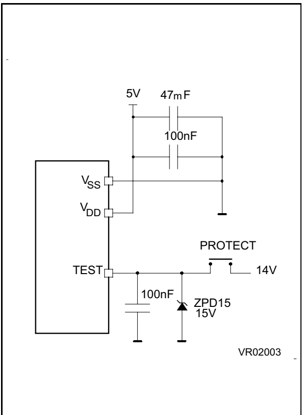
Figure 2. Programming Circuit
