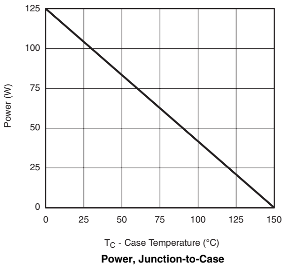
Power, Junction-to-Case
