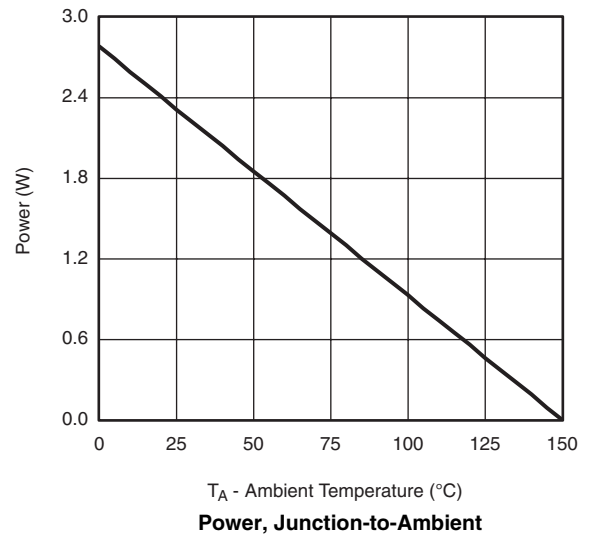
Power, Junction-to-Ambient
