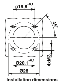
Installation dimensions
