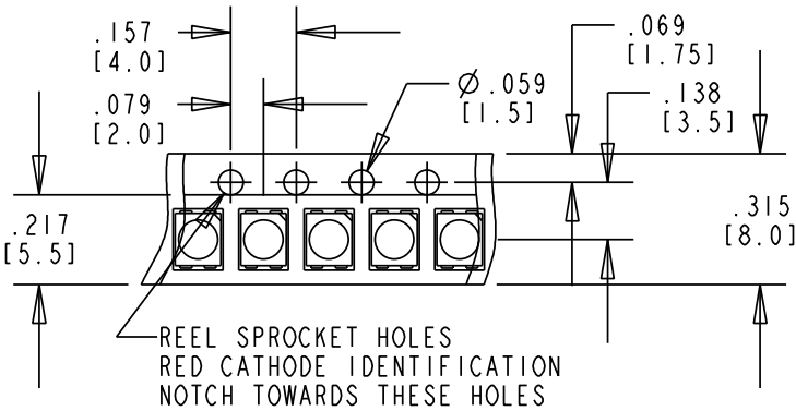
TAPE & REEL CONFIGURATION
