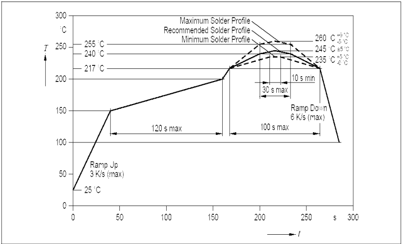
RoHS COMPLIANT REFLOW PROFILE
