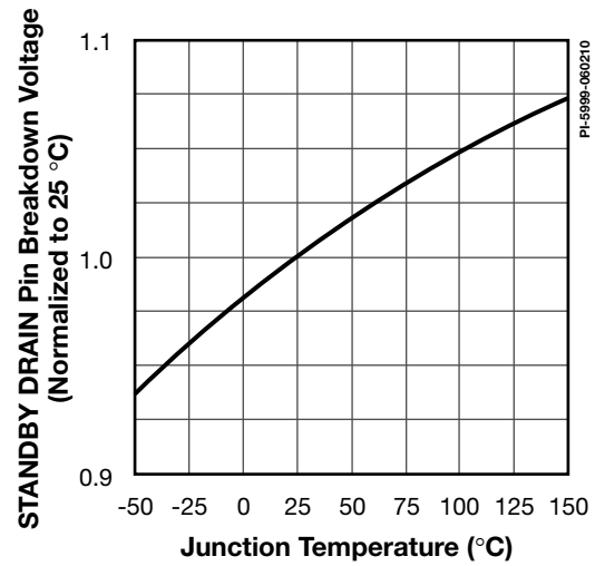
Figure 33. Standby Supply, Breakdown vs. Temperature.
