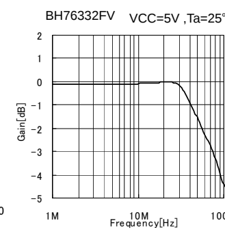
Fig.79 Frequency Response
