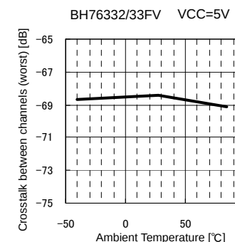
Fig.82 CT(worst) vs. Ambient Temperature
