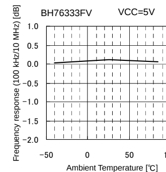
Fig.78 GF vs. Ambient Temperature
