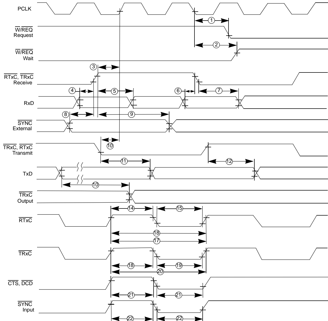
Figure 39. Z80C30 System Timing Diagram
