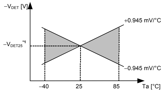
Figure 15 Temperature characteristics of detection voltage ( Example for -V DET = 2.7 V)
