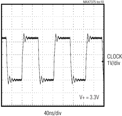
CLOCK OUTPUT WAVEFORM WITH C L = 50pF
