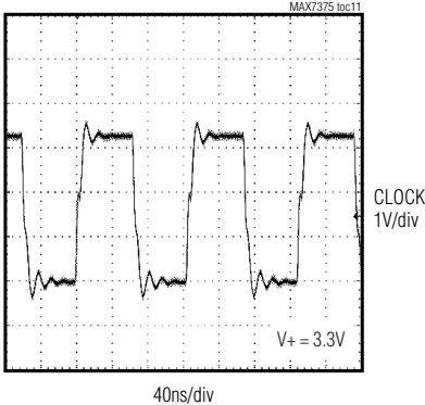
CLOCK OUTPUT WAVEFORM WITH C L = 100pF
