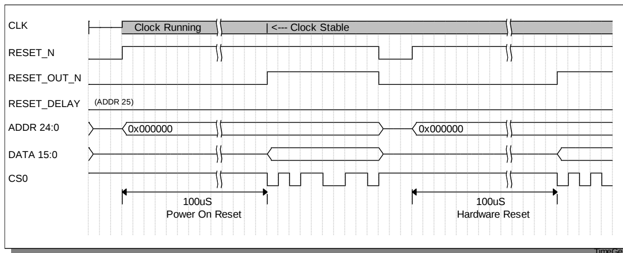
Figure 10. Reset Timing
