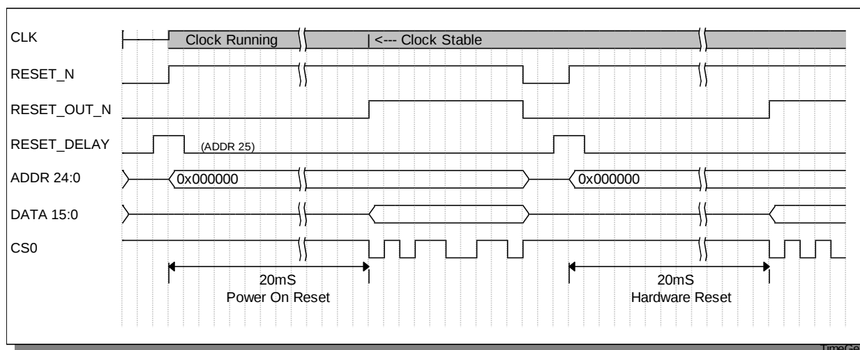
Figure 11. Extended Reset Timing
