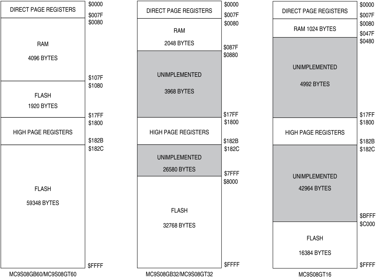
Figure 4-1. MC9S08GB/GT Memory Map
