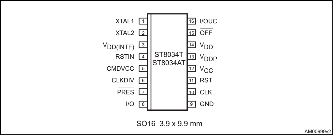
Figure 4. Pin connections ST8034T and ST8034AT, top view
