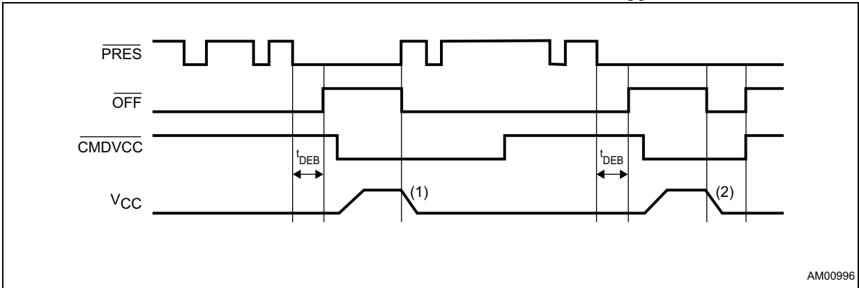
Figure 15. Debounce at \overline{\text{OFF}} , \overline{\text{CMDVCC}} , \overline{\text{PRES}} and V_{CC} pins
