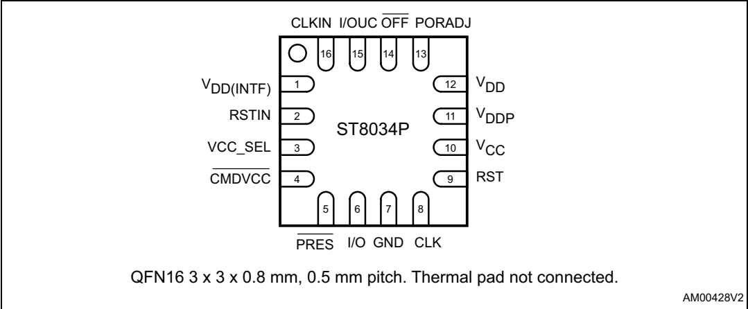
Figure 5. Pin connections ST8034P (options VCC_SEL and PORADJ pins), top-through view
