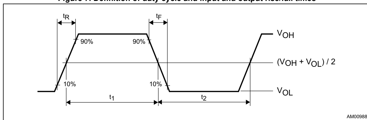
Figure 7. Definition of duty cycle and input and output rise/fall times
