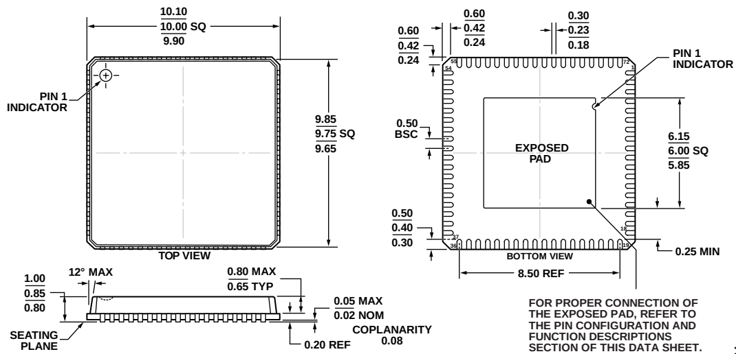
Figure 65. 72-Lead Lead Frame Chip Scale Package [LFCSP_VQ] 10 mm × 10 mm Body, Very Thin Quad (CP-72-7)
