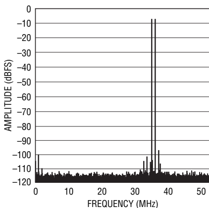
LTC2184: 64k Point 2-Tone FFT, f_{IN} = 69\text{MHz} , 70\text{MHz} , -7\text{dBFS} , 105Mpsps
