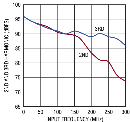
LTC2184: 2nd, 3rd Harmonic vs Input Frequency, -1\text{dBFS} , 105Mpsps, 1V Range
