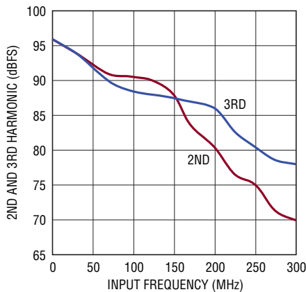
LTC2184: 2nd, 3rd Harmonic vs Input Frequency, -1\text{dBFS} , 105Mpsps, 2V Range
