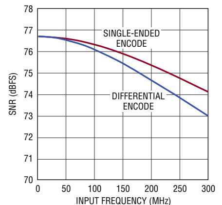
LTC2184: SNR vs Input Frequency, -1\text{dBFS} , 105Mpsps, 2V Range
