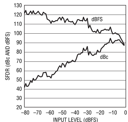
LTC2184: SFDR vs Input Level, f_{IN} = 70\text{MHz} , 105Mpsps, 2V Range
