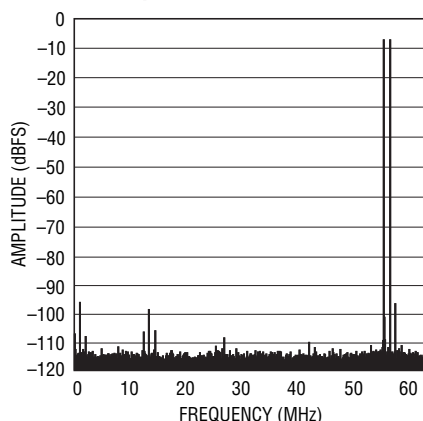
LTC2185: 64k Point 2-Tone FFT, f_{IN} = 69\text{MHz} , 70MHz, -7dBFS, 125Msps
