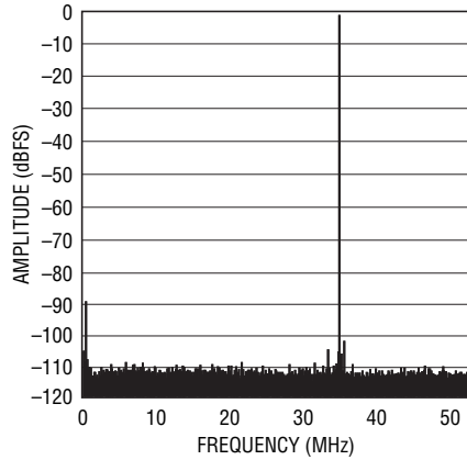
LTC2184: 64k Point FFT, f_{IN} = 70\text{MHz} , -1\text{dBFS} , 105Mpsps
