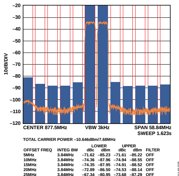
Figure 23. Two-Carrier W-CDMA at 877.5 MHz
