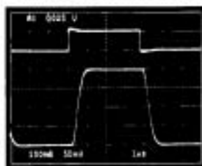
Figure 11. Pulse Response (Small Signal)
