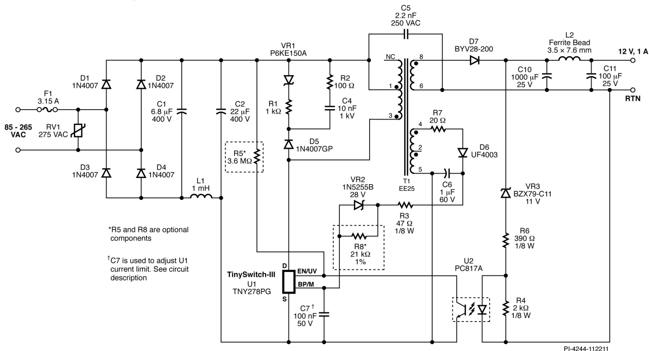
Figure 2 – Schematic.
