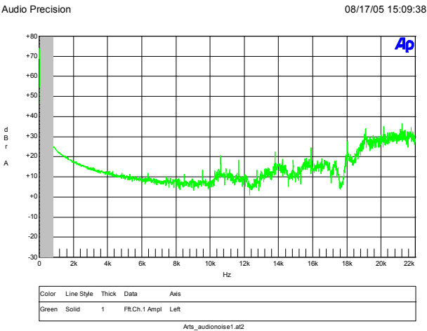
Figure 32 – Audible Noise V_{IN} = 230\text{ VAC} ; I_{OUT} = 1.2\text{ A} .
