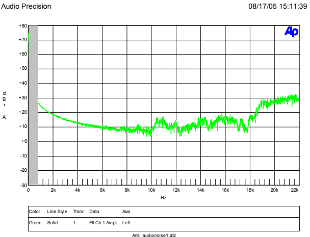
Figure 30 – Audible Noise V_{IN} = 120\text{ VAC} ; I_{OUT} = 1\text{ A} .
