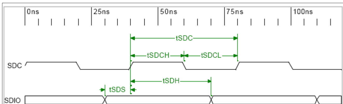
Figure 7 SMI Timing
