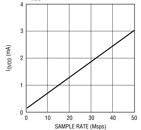
LTC2247: I_{VDD} vs Sample Rate, 5MHz Sine Wave Input, -1dB, O_{VDD} = 1.8\text{V}
