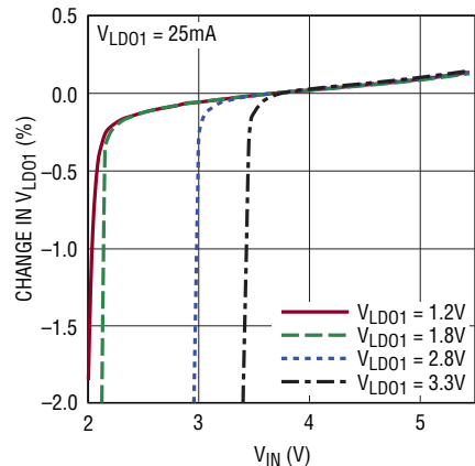
LD01 Output Change vs V_{IN}
