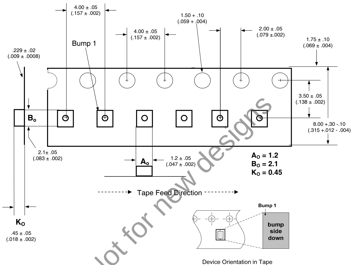
Figure 18. Tape and Reel Specifications
