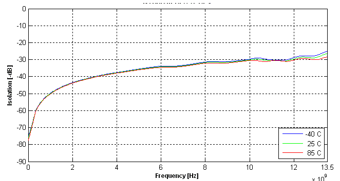
Figure 13. Isolation: RFC to Isolated Port @ 3.3V
