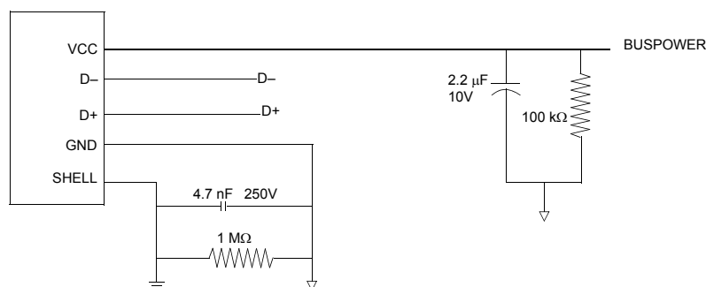
Figure 2. USB Upstream Port Connection
