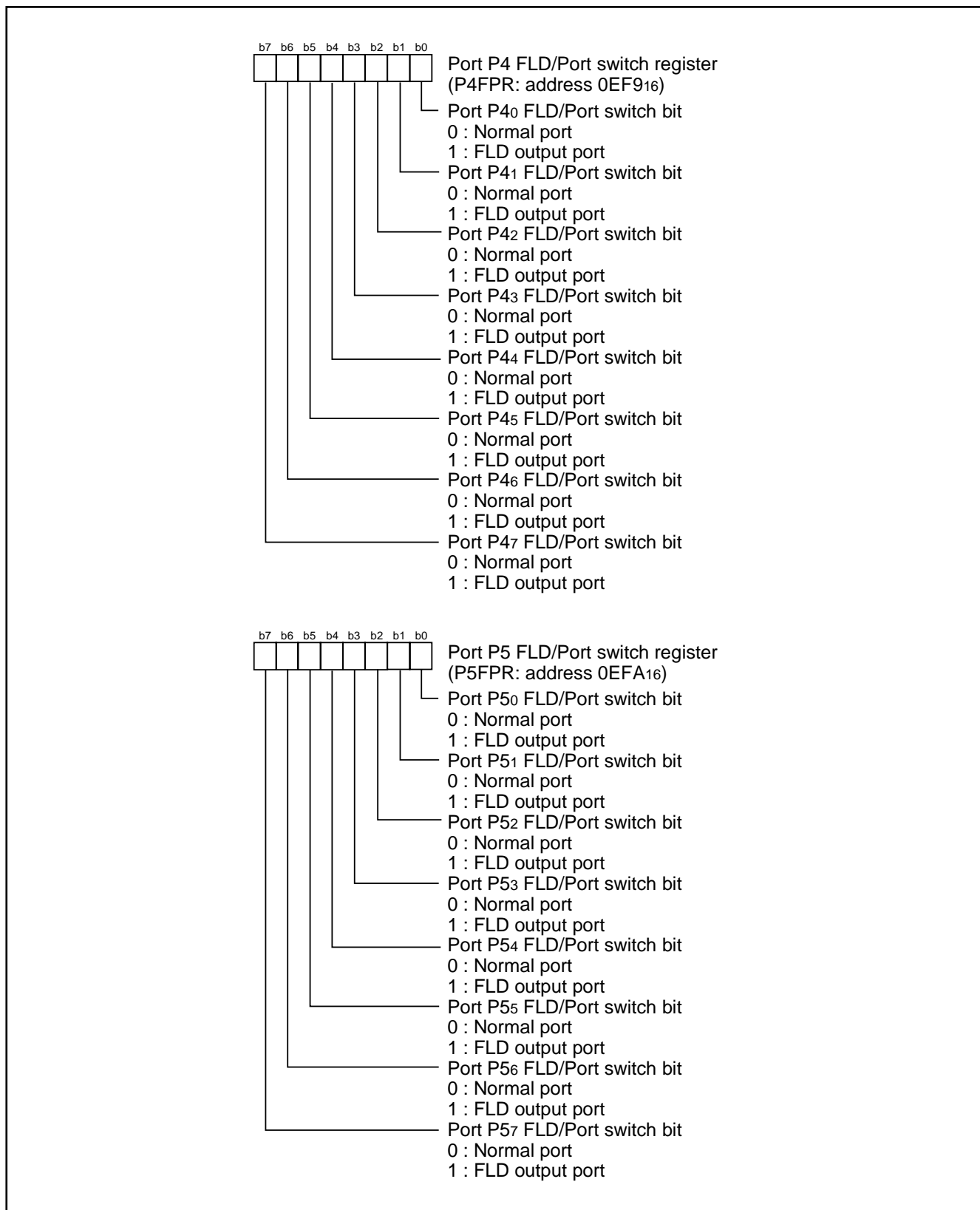
Fig. 46 Structure of FLD-related registers (2)
