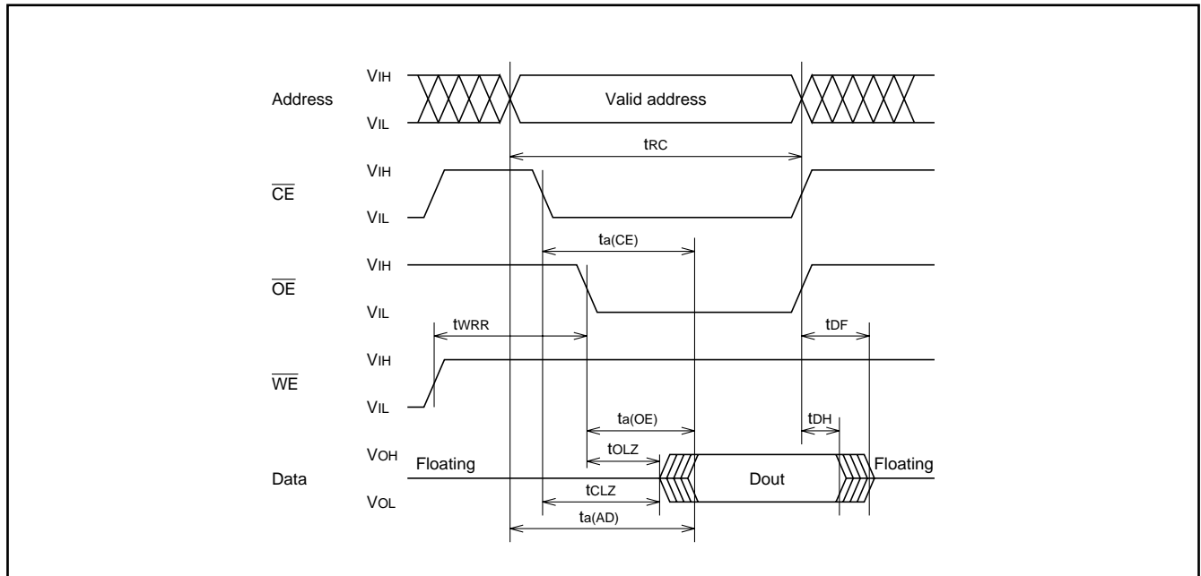
Fig. 86 Read timing
