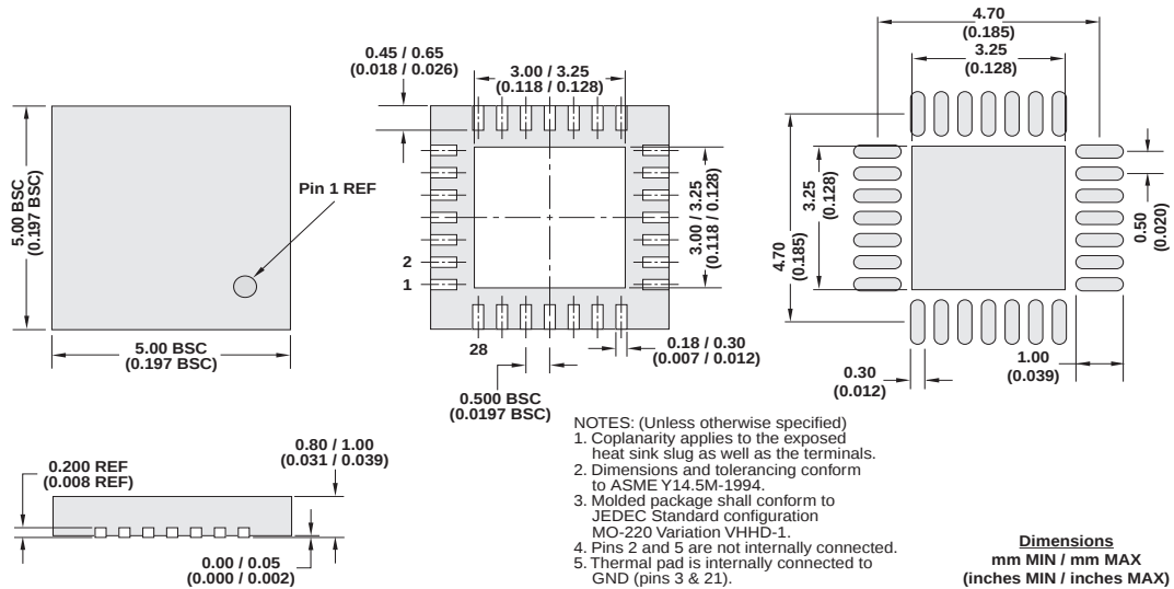
Recommended PCB Land Pattern
