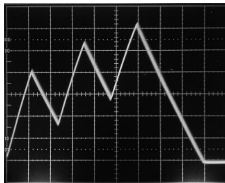
Figure 19. ( I_{LIM} Operation, R_{LIM} = 0 \Omega )
