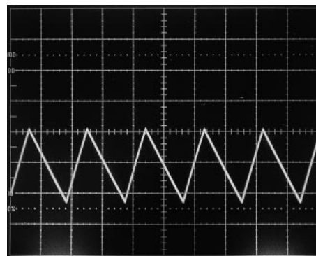
Figure 20. ( I_{IIM} Operation, R_{IIM} = 240 \Omega )
