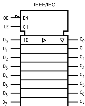
Figure 1. Logic Symbol
