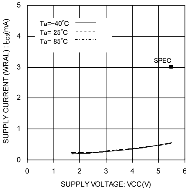
Figure 18. Supply current (WRAL) I_{cc3}(\text{WRAL}, f_{sk}=3\text{MHz})
