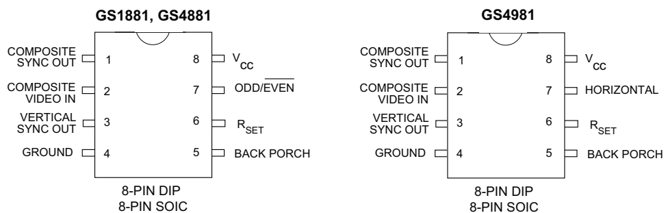
Figure 1-1: 8-Pin DIP, 8-Pin SOIC
