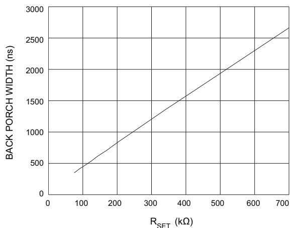
Figure 2-4: Back Porch Width vs R_{SET}
