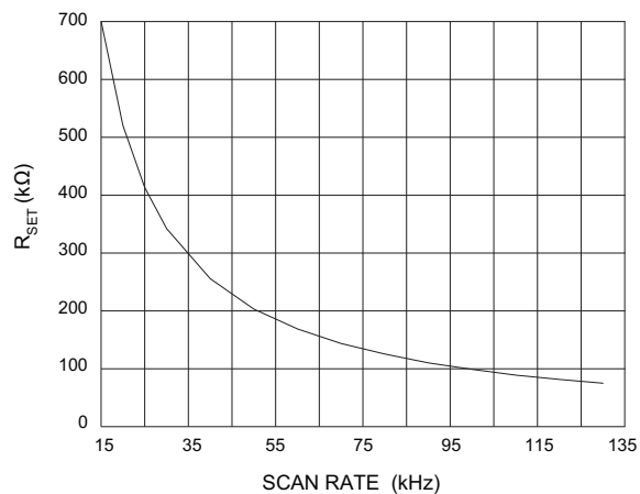
Figure 2-1: R_{SET} vs Scan Rate
