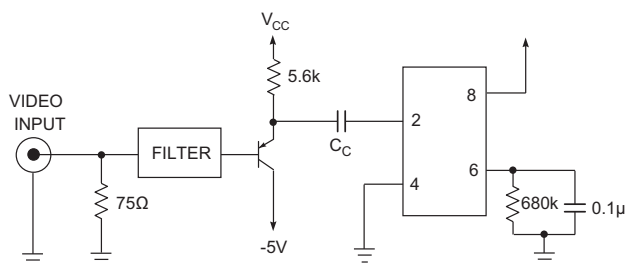
Figure 5-8: PNP Emitter Follower Buffer
