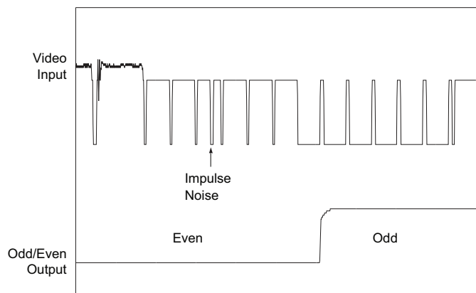
Figure 4-3: Odd/Even Output
