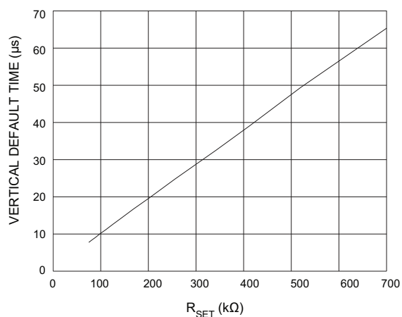
Figure 2-2: Vertical Sync Default Starting Time vs R_{SET}
