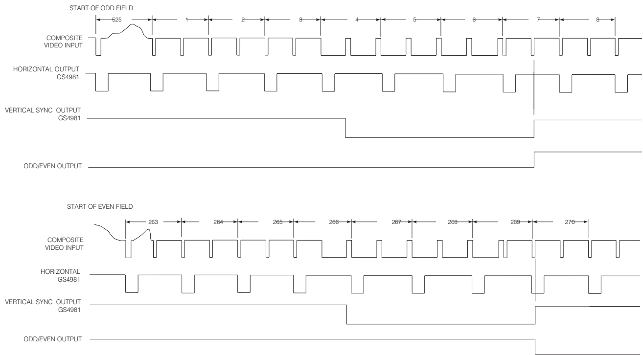
Figure 5-11: Timing Diagram
