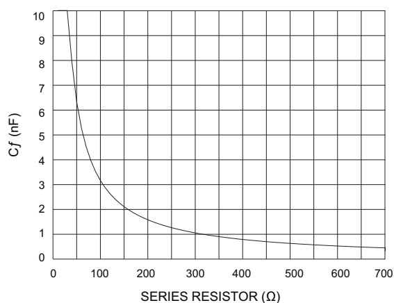
Figure 5-7: C f vs Series Resistor
