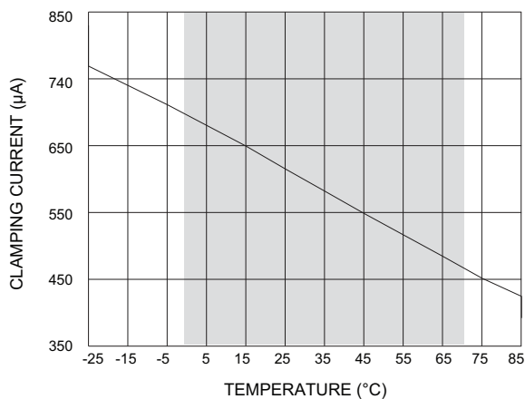
Figure 3-2: Clamping Current vs Temperature
