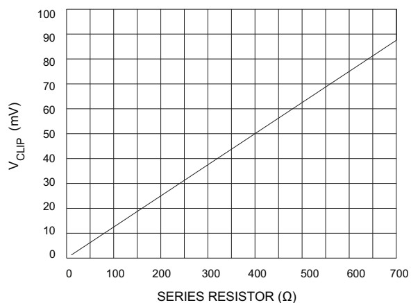
Figure 5-6: V CLIP vs Series Resistor
