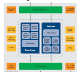
Tsi382A - Block Diagram
