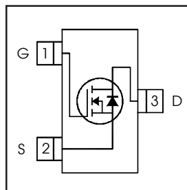
Micro3™ (SOT-23) IRLML6246TRPbF
