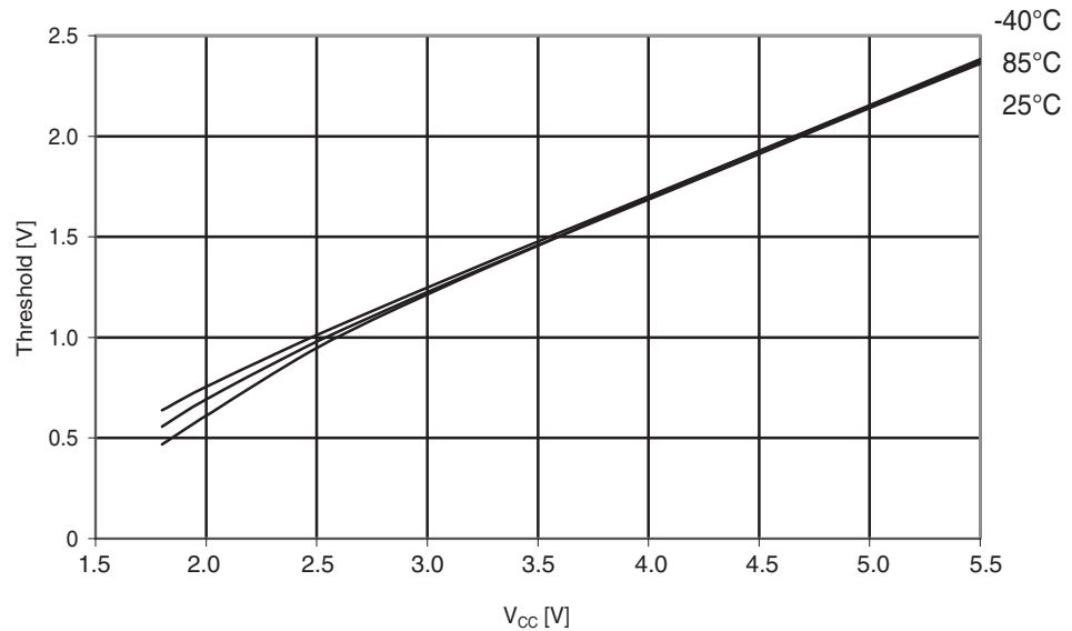
Figure 29-124. Atmel ATmega324A: I/O pin input threshold vs. V_{CC} ( V_{IL} , I/O pin read as '0').
