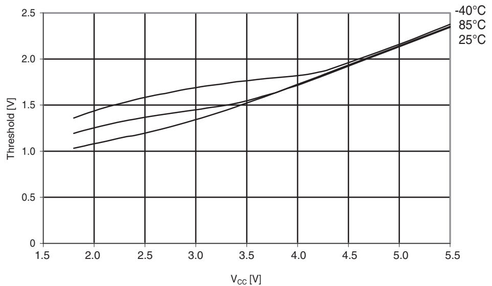
Figure 29-175. Atmel ATmega324PA: Reset pin input threshold vs. V_{CC} ( V_{IH} , I/O pin read as '1').
