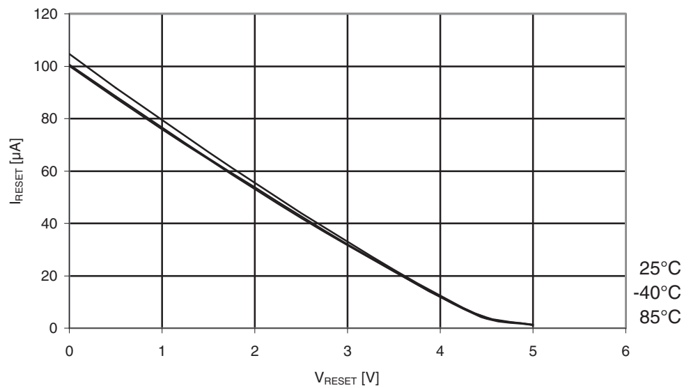
Figure 29-20. Atmel ATmega164A: Reset pull-up resistor current vs. reset pin voltage ( V_{CC} = 5V ).
