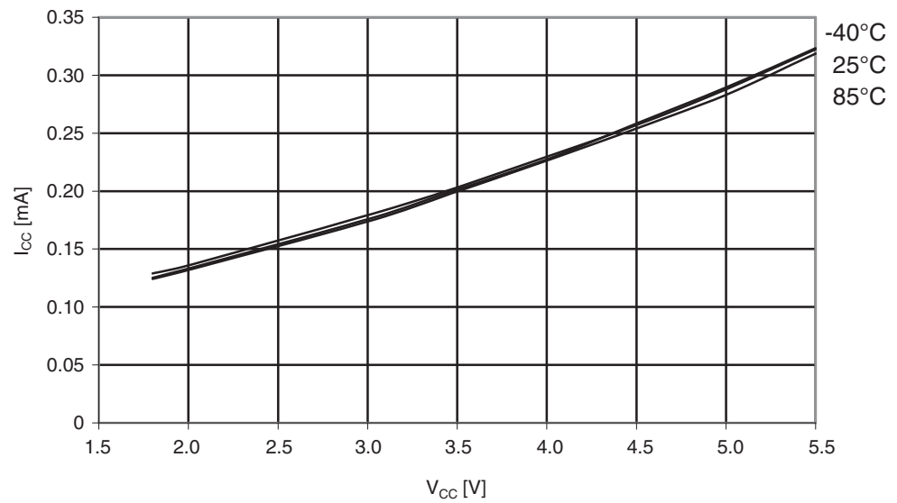
Figure 29-58. Atmel ATmega164PA: Idle supply current vs. V_{CC} (internal RC oscillator, 1MHz).
