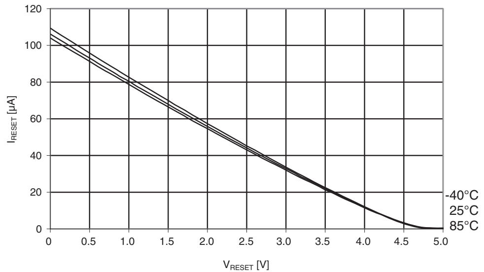
Figure 29-314. Atmel ATmega1284: Reset pull-up resistor current vs. reset pin voltage ( V_{CC} = 5V ).
