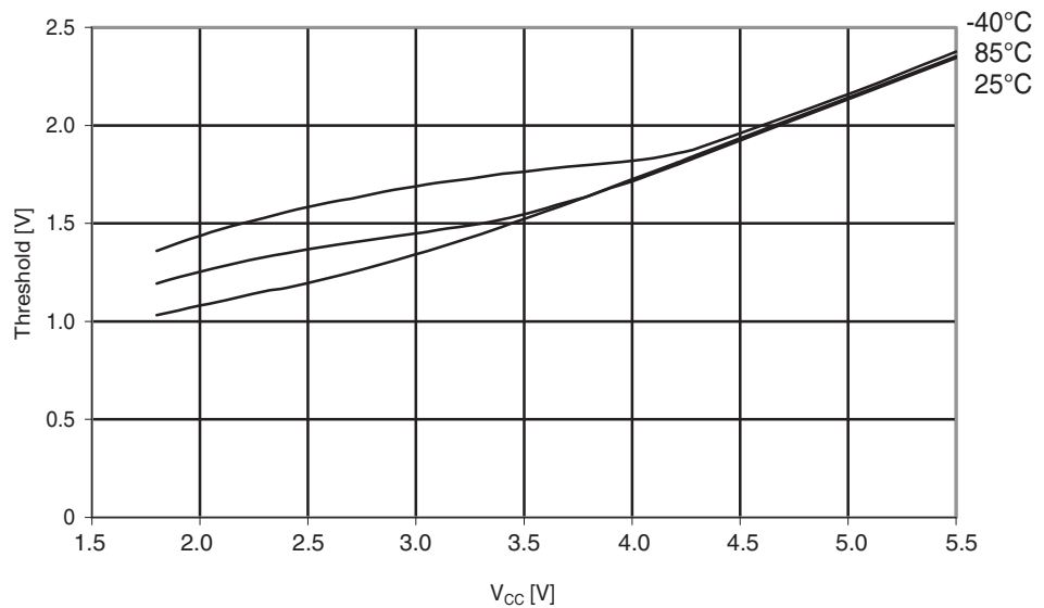
Figure 29-126. Atmel ATmega324A: Reset pin input threshold vs. V_{CC} ( V_{IH} , I/O pin read as '1').
