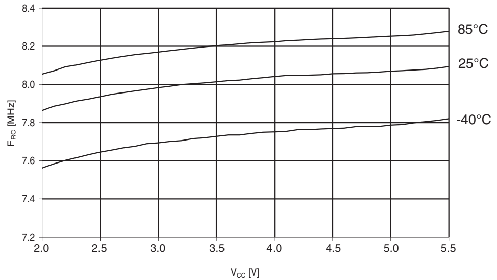
Figure 29-234. Atmel ATmega644A: Calibrated 8MHz RC oscillator vs. V_{CC} .
