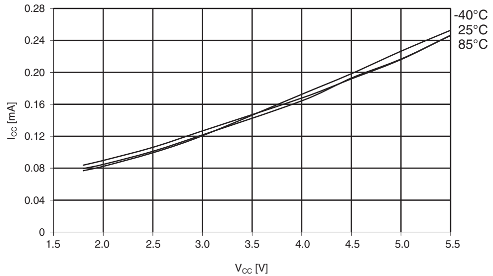
Figure 29-349. Atmel ATmega1284P: Active supply current vs. V_{CC} (internal RC oscillator, 128kHz).
