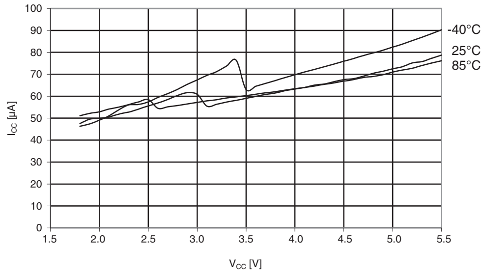
Figure 29-42. Atmel ATmega164A: Analog comparator current vs. V_{CC} .
