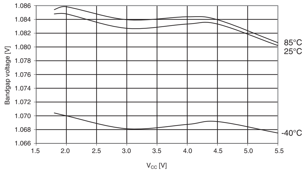
Figure 29-279. Atmel ATmega644PA: Calibrated bandgap voltage vs. V_{CC} .
