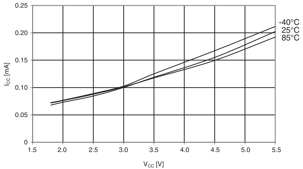
Figure 29-5. Atmel ATmega164A: Active supply current vs. V_{CC} (internal RC oscillator, 128kHz).
