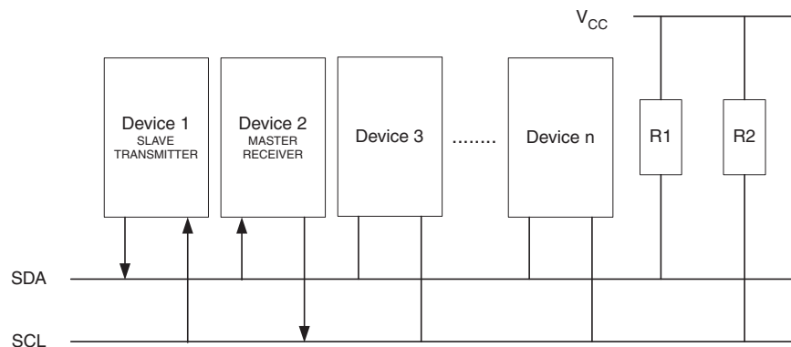
Figure 21-17. Data transfer in Slave Transmitter mode.
