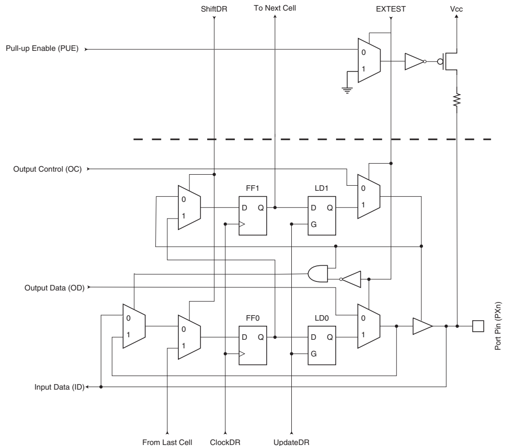
Figure 25-3. Boundary-scan cell for bi-directional port pin with pull-up function.
