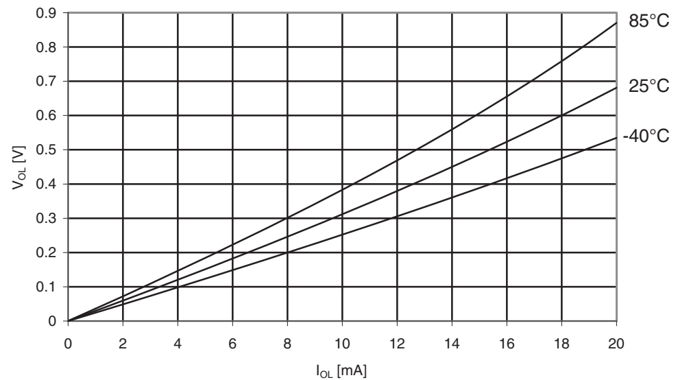
Figure 29-366. Atmel ATmega1284P: I/O pin output voltage vs. sink current ( V_{CC} = 3V ).
