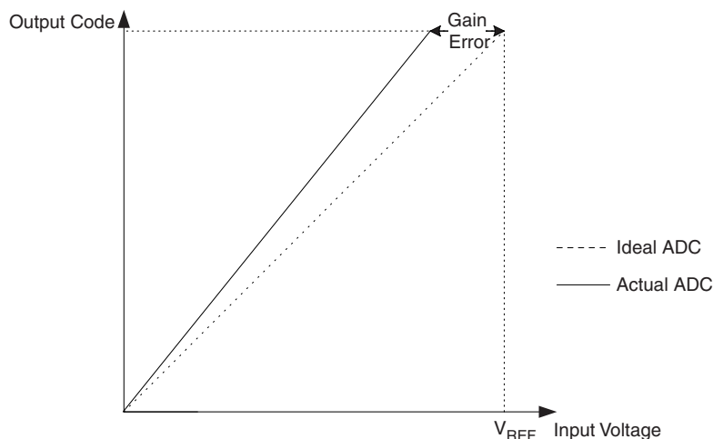
Figure 23-11. Gain error.
