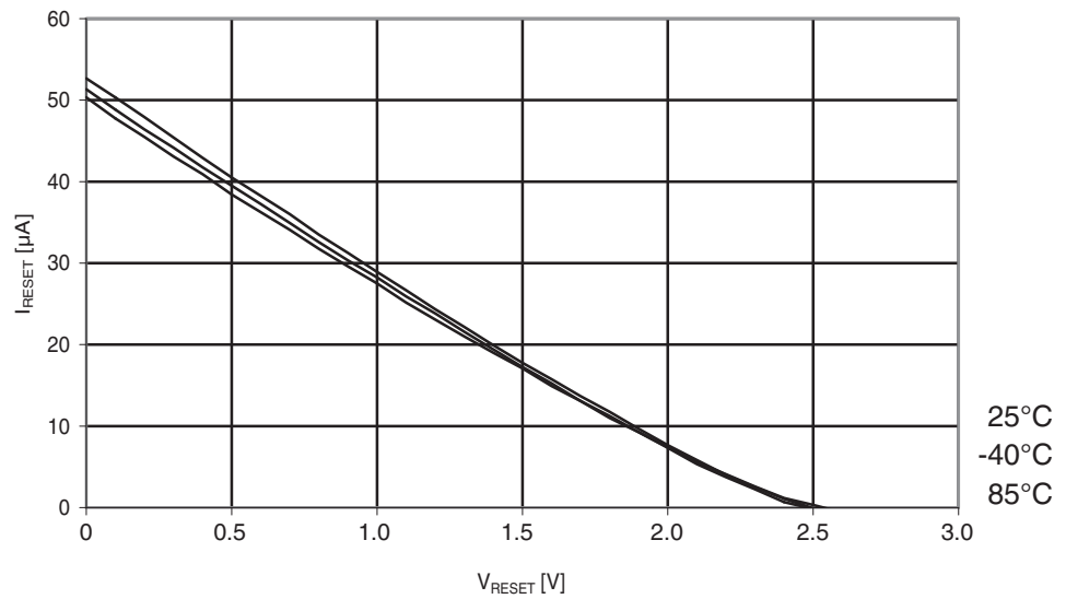
Figure 29-265. Atmel ATmega644PA: Reset pull-up resistor current vs. reset pin voltage ( V_{CC} = 5V ).
