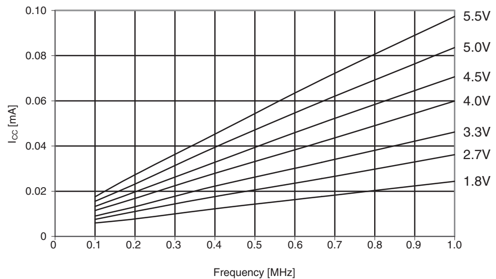
Figure 29-342. Atmel ATmega1284: Reset supply current vs. low frequency (0.1 - 1.0MHz).
