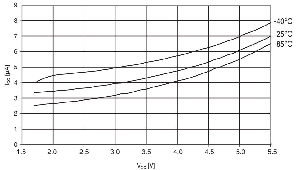
Figure 29-242. Atmel ATmega644A: Watchdog timer current vs. V_{CC} .
