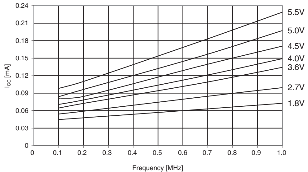
Figure 29-350. Atmel ATmega1284P: Idle supply current vs. low frequency (0.1 - 1.0MHz).
