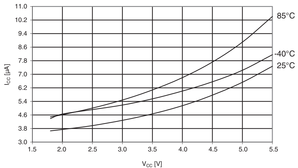
Figure 29-306. Atmel ATmega1284: Power-down supply current vs. V_{CC} (watchdog timer enabled).
