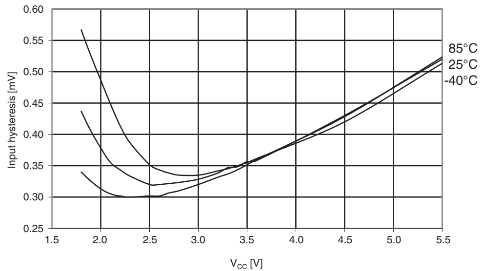
Figure 29-372. Atmel ATmega1284P: I/O pin input hysteresis vs. V_{CC} .
