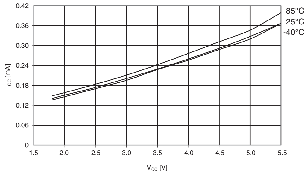
Figure 29-303. Atmel ATmega1284: Idle supply current vs. V_{CC} (internal RC oscillator, 1MHz).
