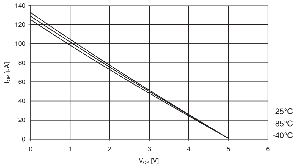
Figure 29-17. Atmel ATmega164A: I/O pin pull-up resistor current vs. input voltage ( V_{CC} = 5V ).
