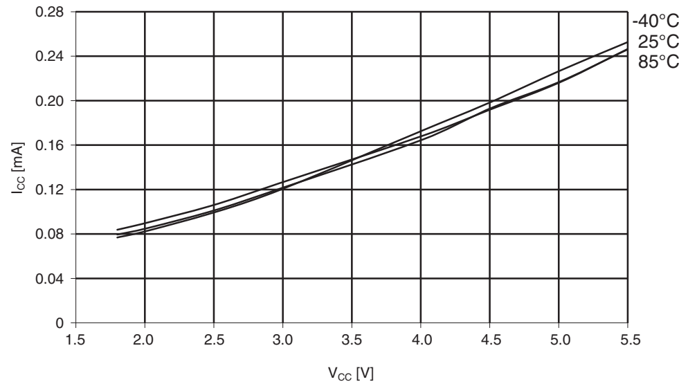
Figure 29-299. Atmel ATmega1284: Active supply current vs. V_{CC} (internal RC oscillator, 128kHz).
