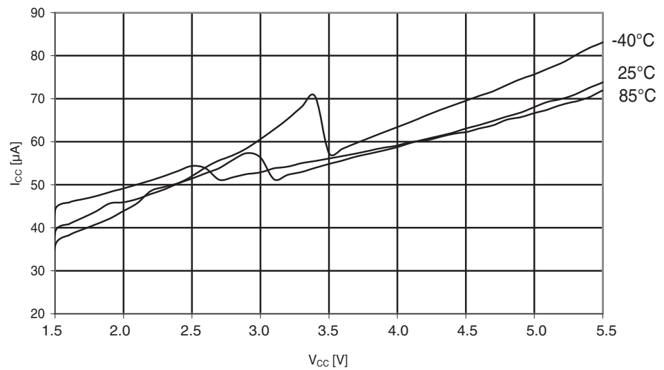
Figure 29-287. Atmel ATmega644PA: Analog comparator current vs. V_{CC} .
