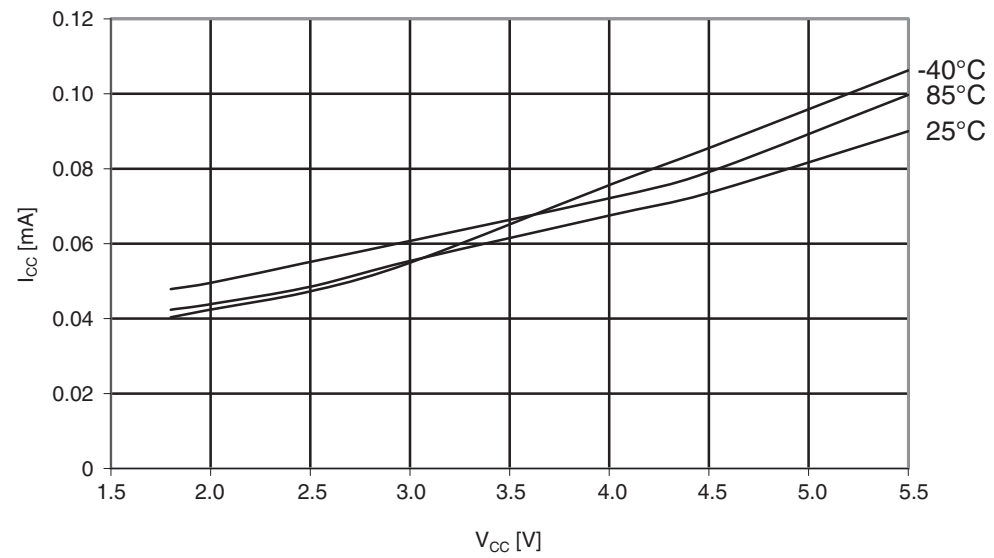
Figure 29-304. Atmel ATmega1284: Idle supply current vs. V_{CC} (internal RC oscillator, 128kHz).
