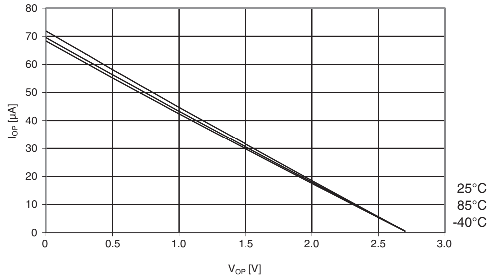
Figure 29-65. Atmel ATmega164PA: I/O pin pull-up resistor current vs. input voltage ( V_{CC} = 2.7V ).
