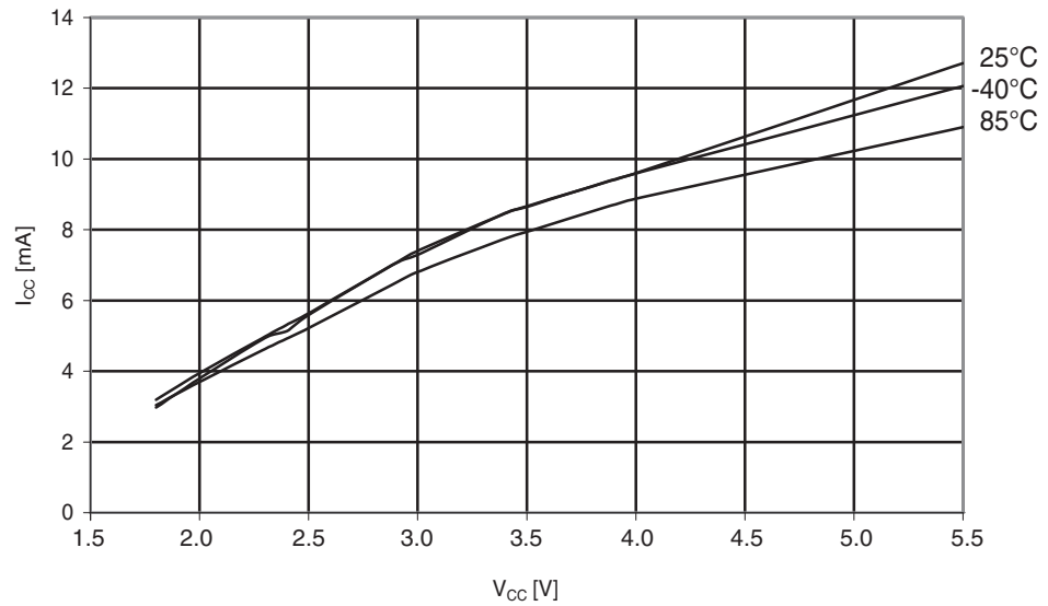
Figure 29-143. Atmel ATmega324A: Programming current vs. V_{CC} .
