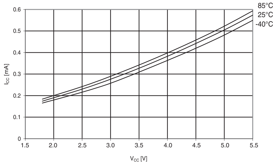
Figure 29-107. Atmel ATmega324A: Idle supply current vs. V_{CC} (internal RC oscillator, 1MHz).
