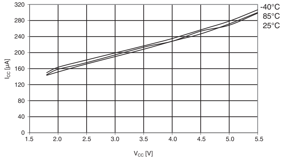
Figure 29-90. Atmel ATmega164PA: ADC current vs. V_{CC} ( A_{REF} = A_{V_{CC}} ).
