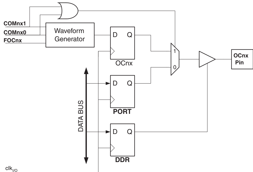
Figure 16-5. Compare Match Output unit, schematic.
