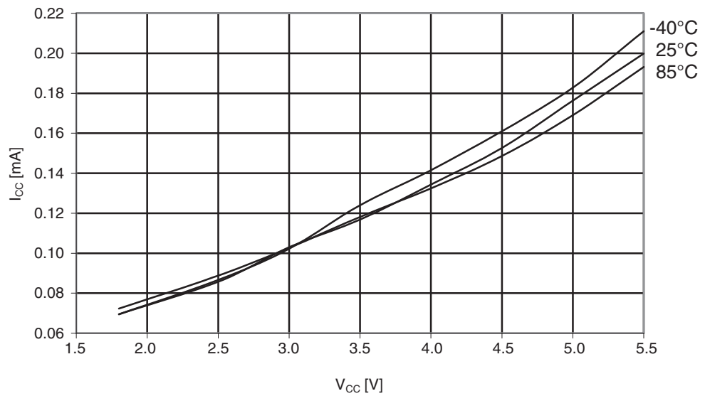
Figure 29-250. Atmel ATmega644PA: Active supply current vs. V_{CC} (internal RC oscillator, 128kHz).
