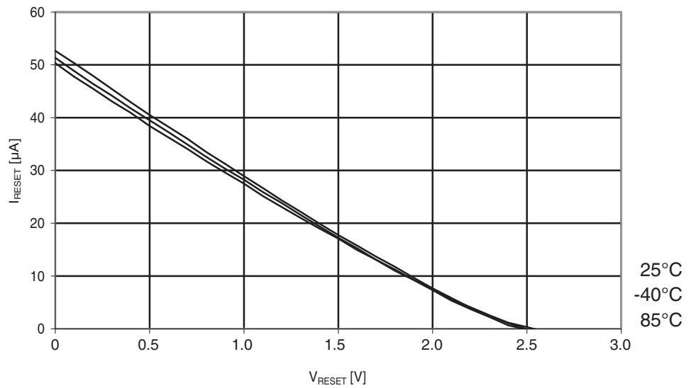
Figure 29-216. Atmel ATmega644A: Reset pull-up resistor current vs. reset pin voltage ( V_{CC} = 5V ).
