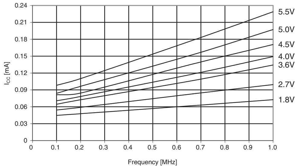
Figure 29-300. Atmel ATmega1284: Idle supply current vs. low frequency (0.1 - 1.0MHz).
