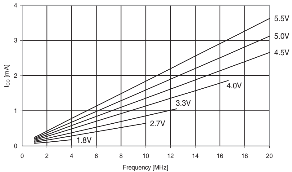
Figure 29-154. Atmel ATmega324PA: Idle supply current vs. V_{CC} (1 - 20MHz).
