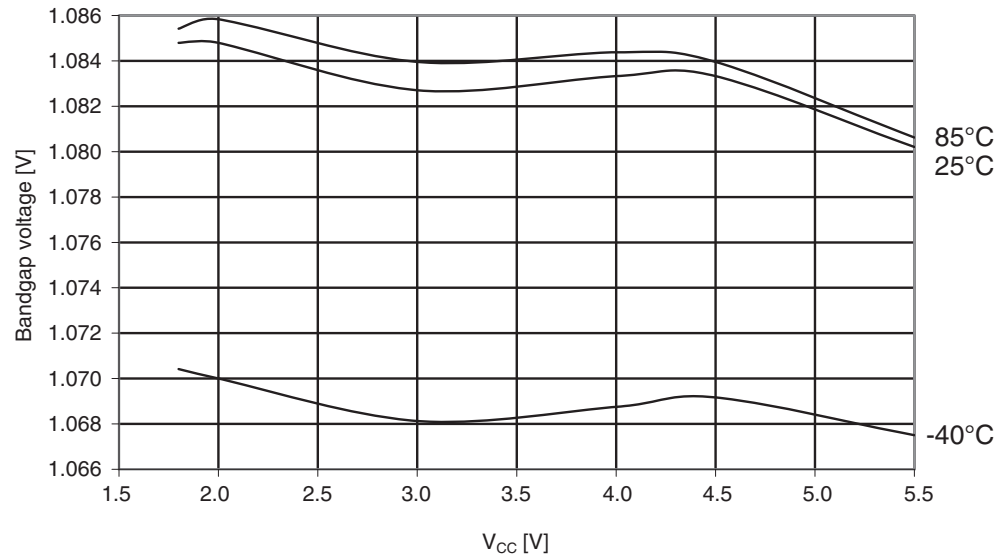
Figure 29-230. Atmel ATmega644A: Calibrated bandgap voltage vs. V_{CC} .
