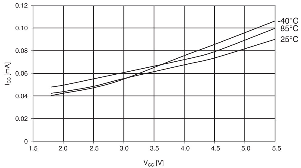
Figure 29-354. Atmel ATmega1284P: Idle supply current vs. V_{CC} (internal RC oscillator, 128kHz).
