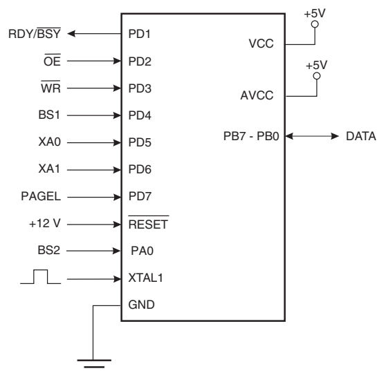
Figure 27-1. Parallel programming (1) .
