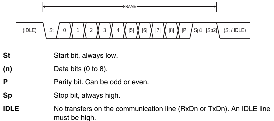
Figure 19-4. Frame formats.
