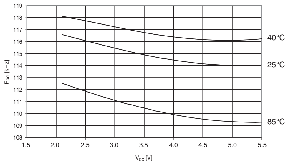
Figure 29-282. Atmel ATmega644PA: Watchdog oscillator frequency vs. V_{CC} .
