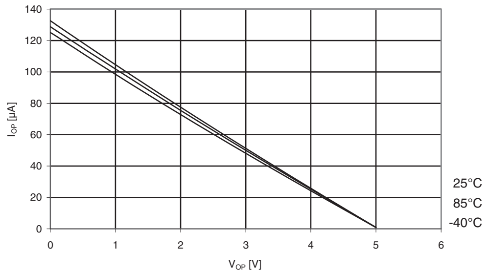
Figure 29-66. Atmel ATmega164PA: I/O pin pull-up resistor current vs. input voltage ( V_{CC} = 5V ).
