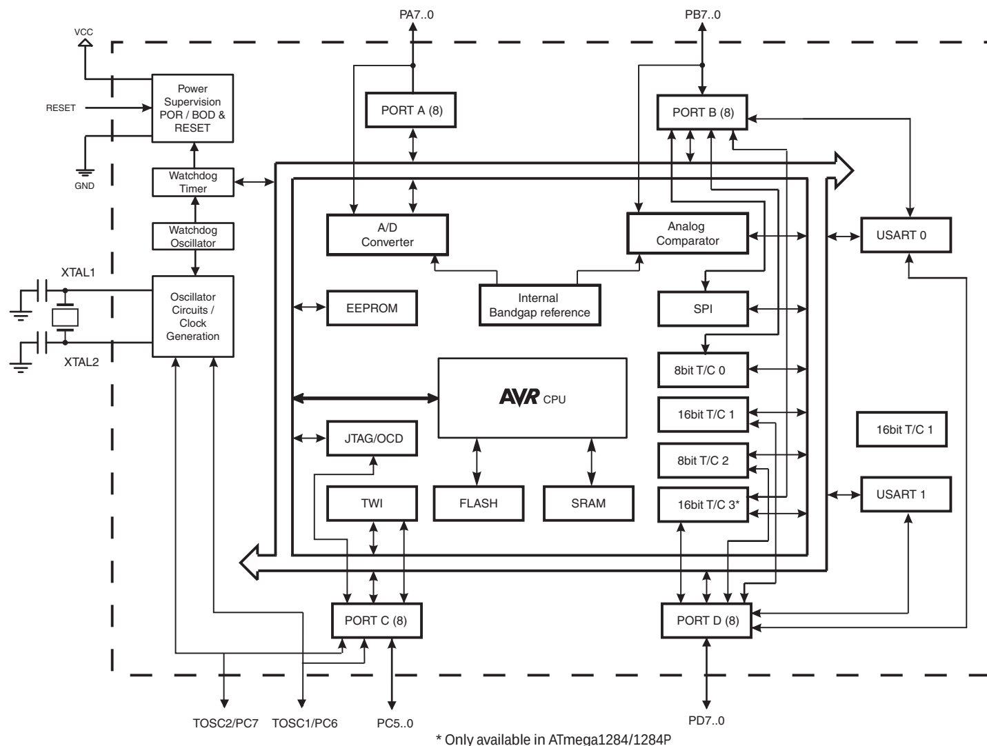
Figure 2-1. Block diagram.
