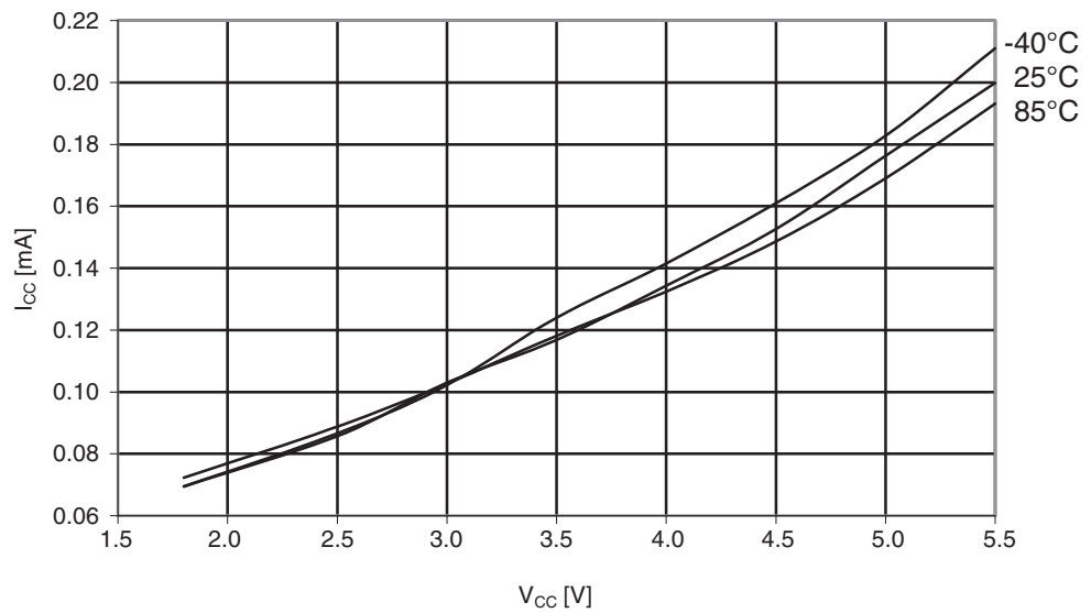
Figure 29-201. Atmel ATmega644A: Active supply current vs. V_{CC} (internal RC oscillator, 128kHz).
