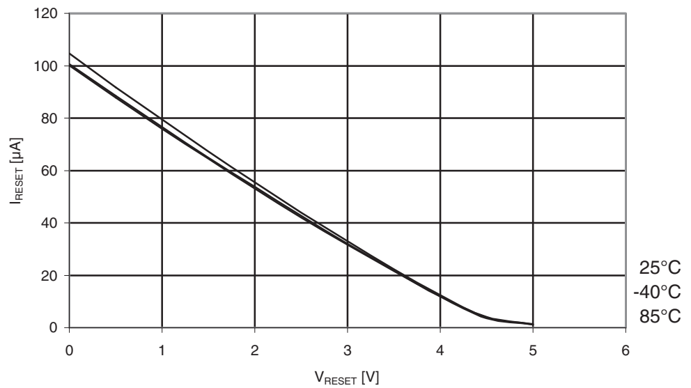
Figure 29-69. Atmel ATmega164PA: Reset pull-up resistor current vs. reset pin voltage ( V_{CC} = 5V ).
