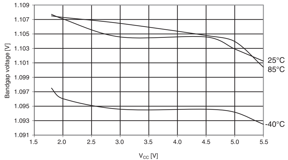
Figure 29-34. Atmel ATmega164A: Calibrated bandgap voltage vs. V_{CC} .
