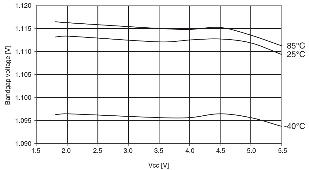
Figure 29-379. Atmel ATmega1284P: Calibrated bandgap voltage vs. V_{CC} .
