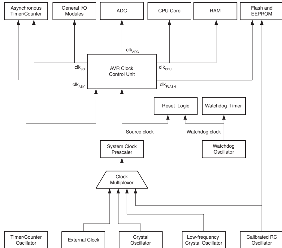
Figure 9-1. Clock distribution.
