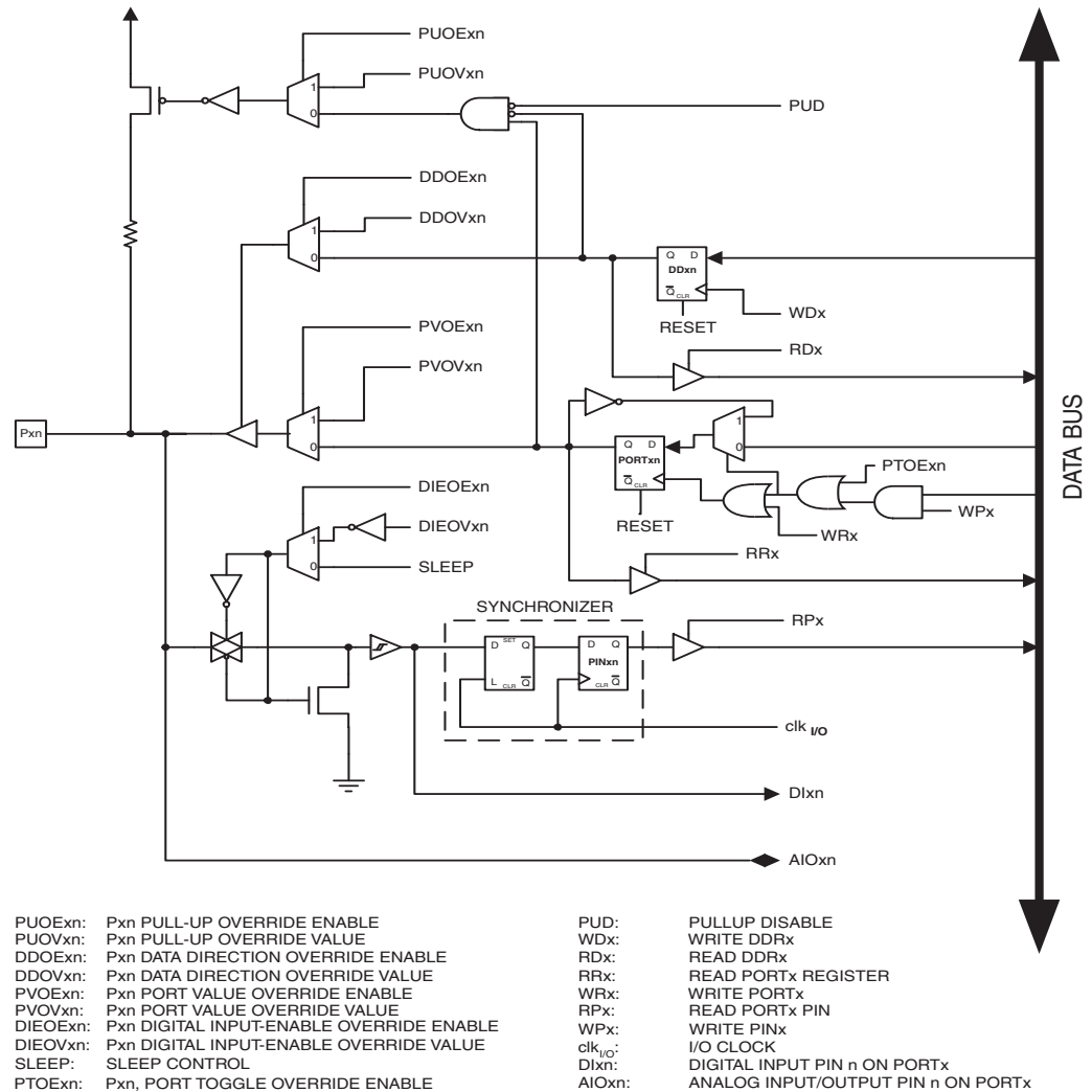
Figure 14-5. Alternate port functions (1) .
