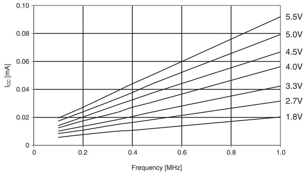
Figure 29-47. Atmel ATmega164A: Reset supply current vs. low frequency (0.1 - 1.0MHz).
