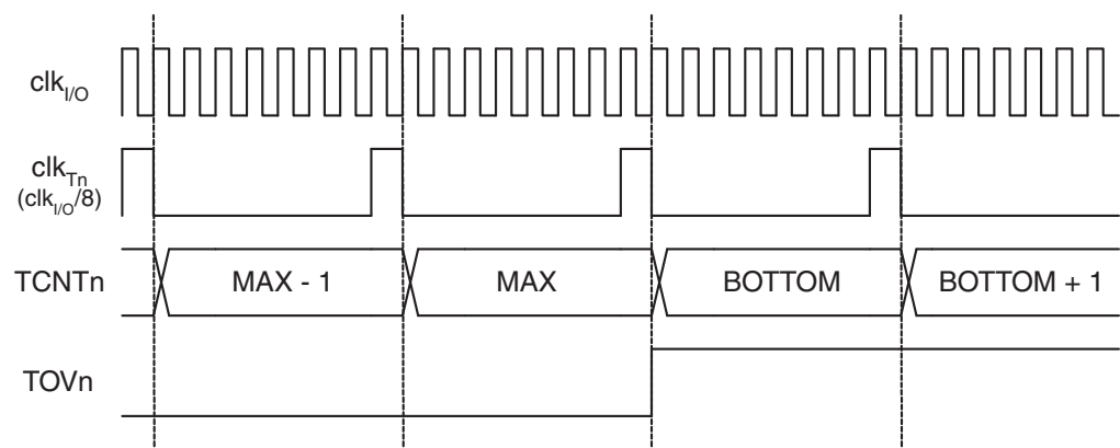
Figure 17-9. Timer/Counter Timing diagram, with prescaler ( f_{clk_{I/O}}/8 ).
