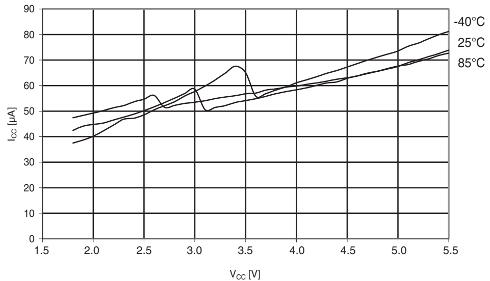
Figure 29-140. Atmel ATmega324A: Analog comparator current vs. V_{CC} .
