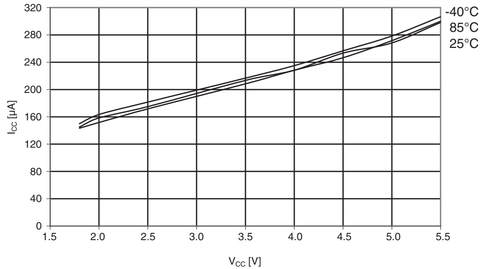
Figure 29-41. Atmel ATmega164A: ADC current vs. V_{CC} ( AREF = AV_{CC} ).
