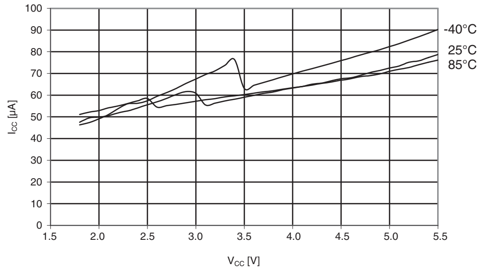
Figure 29-91. Atmel ATmega164PA: Analog comparator current vs. V_{CC} .
