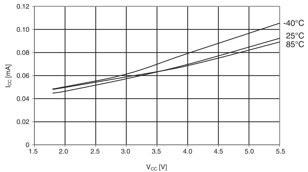
Figure 29-10. Atmel ATmega164A: Idle supply current vs. V_{CC} (internal RC oscillator, 128kHz).
