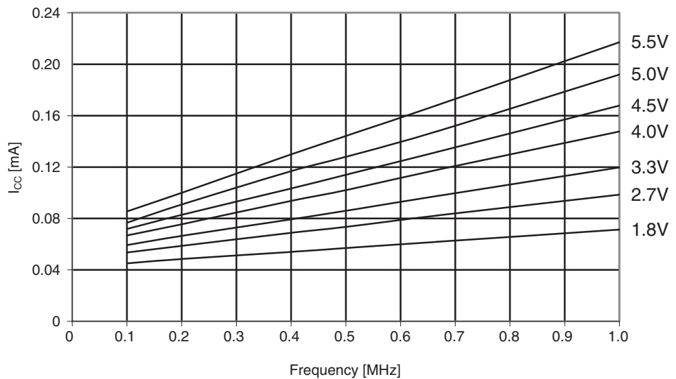
Figure 29-202. Atmel ATmega644A: Idle supply current vs. V_{CC} (0.1 - 1.0MHz).
