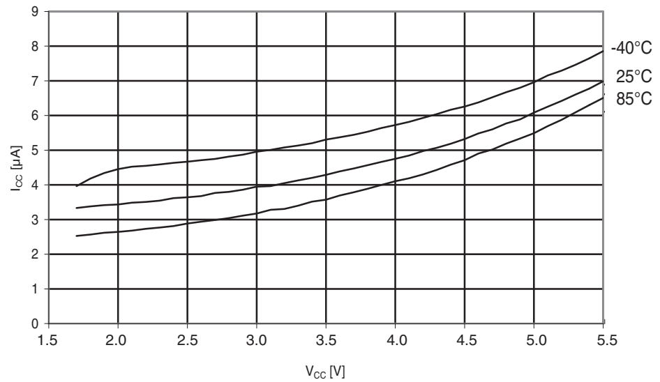
Figure 29-291. Atmel ATmega644PA: Watchdog timer current vs. V_{CC} .
