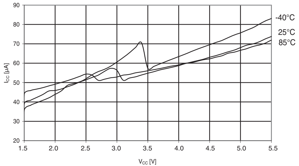
Figure 29-238. Atmel ATmega644A: Analog comparator current vs. V_{CC} .
