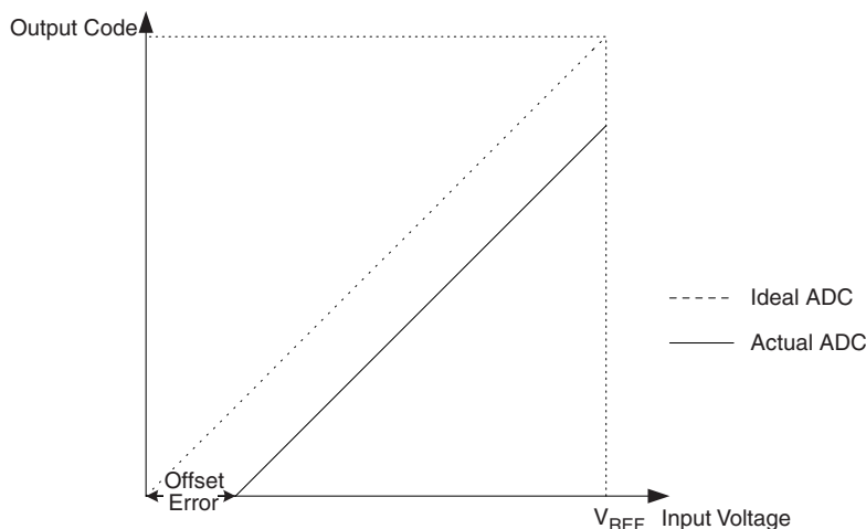
Figure 23-10. Offset error.
