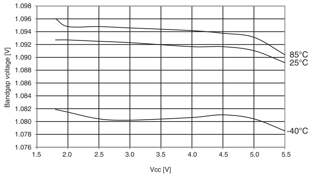
Figure 29-132. Atmel ATmega324A: Calibrated bandgap voltage vs. V_{CC} .
