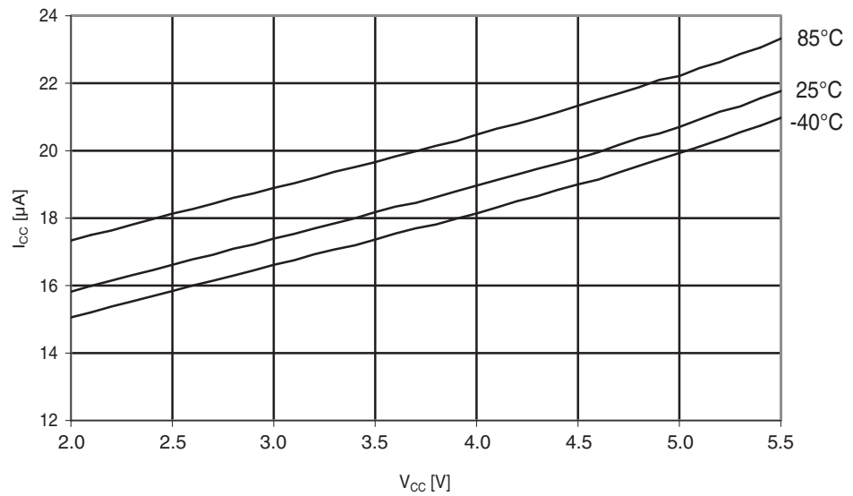
Figure 29-289. Atmel ATmega644PA: Brownout detector current vs. V_{CC} .
