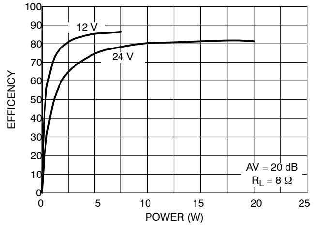
Figure 11. Efficiency vs. P_{\text{out}}
