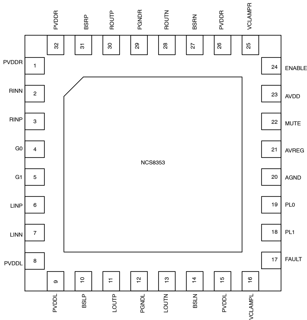
Figure 2. Package Options
