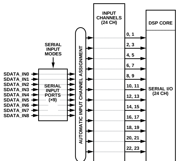
Figure 40. Input Routing in the ADAU1446
