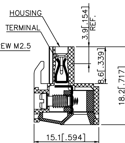
SECTION P-P
