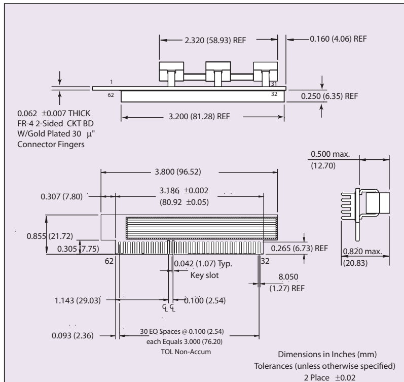
Figure 1: Mechanical Drawing
