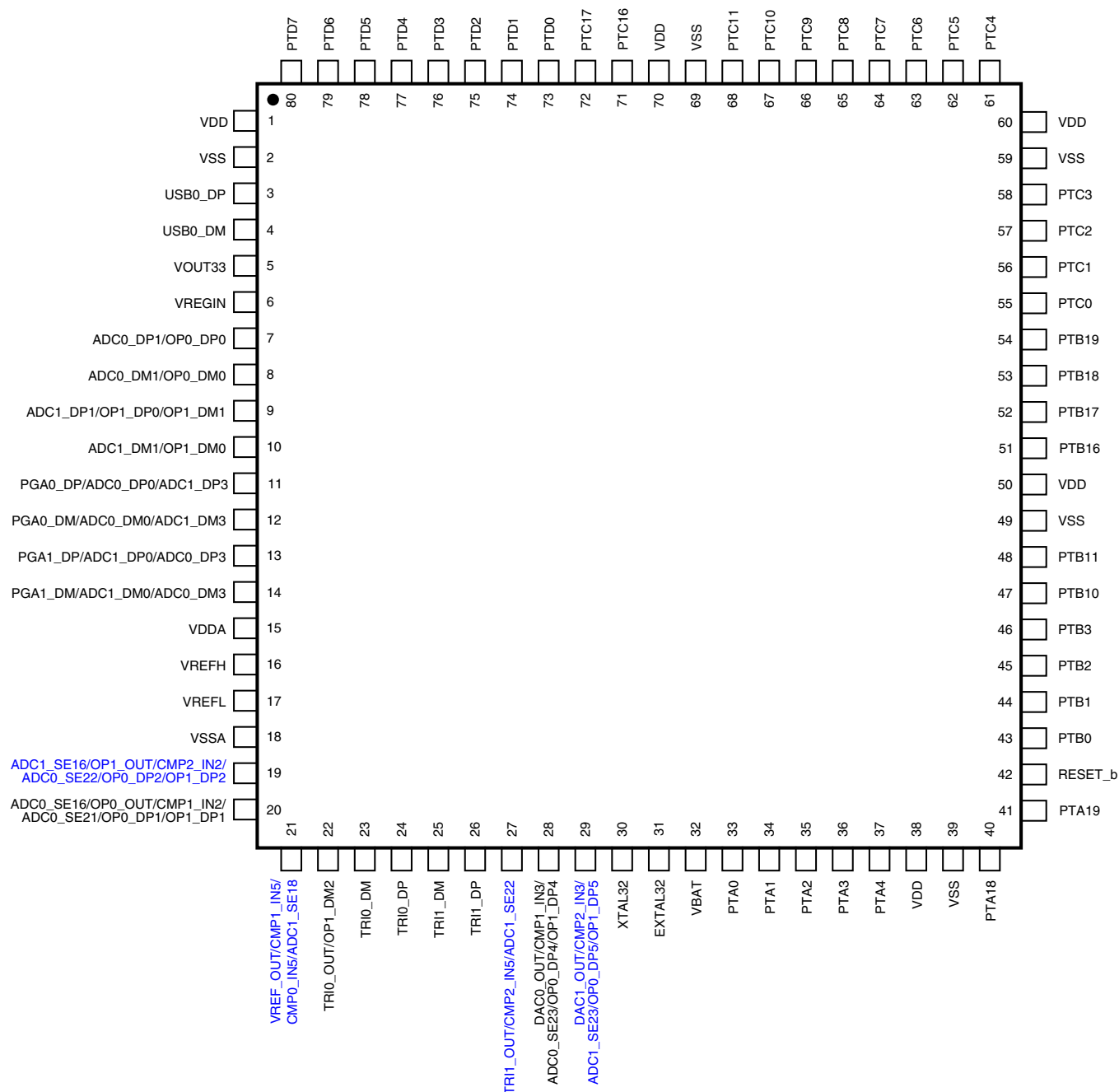
Figure 28. K50 80 LQFP Pinout Diagram
