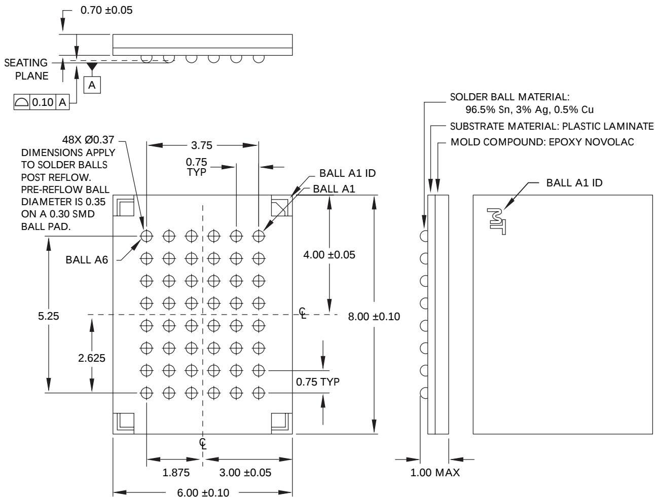
Figure 24: 48-Ball VFBGA
