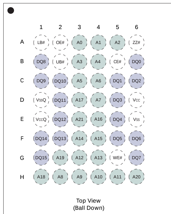
Figure 1: 48-Ball VFBGA Ball Assignment
