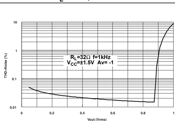
Figure 10. THD + noise vs. output voltage, R_L = 32\ \Omega , f = 1\text{ kHz}
