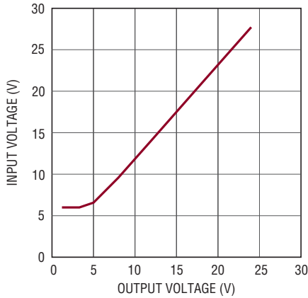
Minimum Required Input Running Voltage vs Output Voltage, I_{OUT} = 5\text{A}
